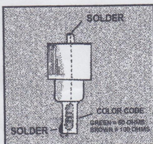
Figure 1 Terminator Plug
