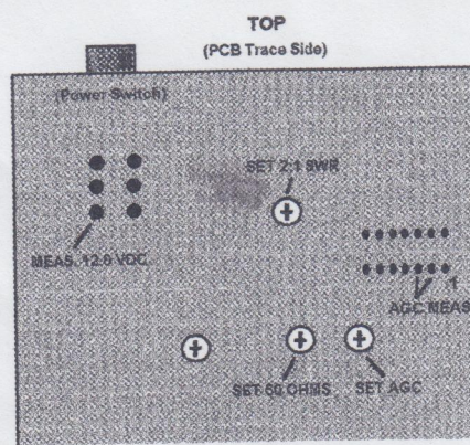
Figure 2. PCB Locator
